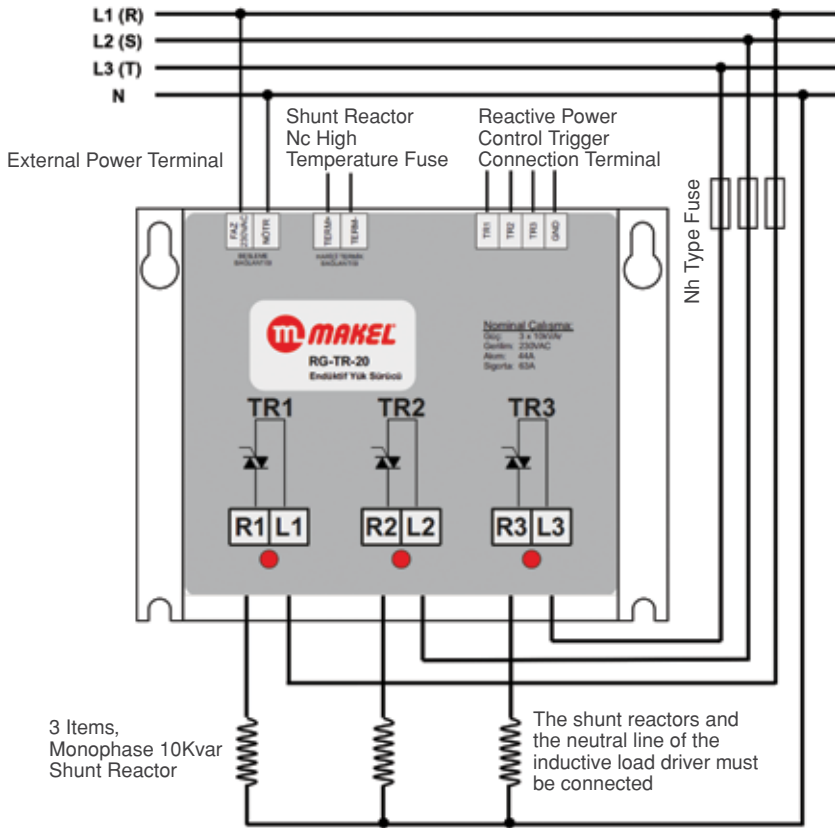
RG-TR-30-Diagram
